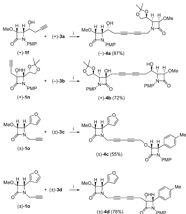
Scheme 4. Copper-promoted preparation of unsymmetrical bis( \beta -lactam)-1,3-diynes 4a–d . Reagents and conditions: (i) MeOH/ \text{CH}_2\text{Cl}_2 , CuCl, \text{NH}_2\text{OH}\cdot\text{HCl} , \text{EtNH}_2 , 0 °C; 4a : 3 h; 4b : 3 h; 4c : 4 h; 4d : 2 h.
