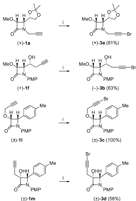
Scheme 3. Preparation of bromoalkynyl-β-lactams 3 . Reagents and conditions: (i) NBS, AgOAc (or AgNO 3 ), acetone, room temp., darkness; 3a : 3 h; 3b : 2.5 h; 3c : 21 h; 3d : 4 h.
