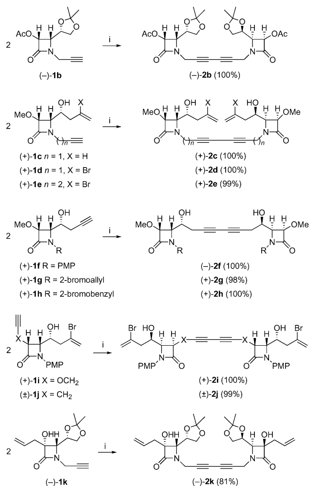
Scheme 2. Copper-promoted preparation of C 2 -symmetrical bis(β-lactam)-1,3-diynes 2b–k . Reagents and conditions: (i) Cu(OAc) 2 , K 2 CO 3 , MeCN, room temp.; 2b : 5 h; 2c : 22 h; 2d : 6 h; 2e : 2 h; 2f : 168 h; 2g : 6 h; 2h : 20 h; 2i : 16 h; 2j : 18 h; 2k : 24 h.
