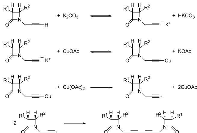
Scheme 6. Mechanistic explanation for the Cu-promoted homocoupling of alkynyl- \beta -lactams by using \text{Cu}(\text{OAc})_2 and \text{K}_2\text{CO}_3 in the absence of \text{O}_2 .
