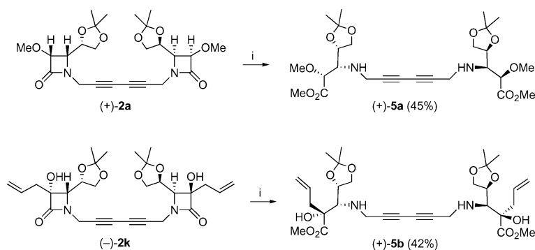
Scheme 5. Preparation of bis( \beta -amino ester)-1,3-diynes 5 . Reagents and conditions: (i) MeONa, MeOH, sealed tube, 65 °C; 5a : 1 h; 5b : 8 h.
