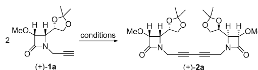
Scheme 1. Homocoupling reaction of N -alkynyl-2-azetidinone (+)- 1a .
